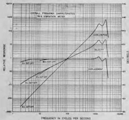
FIGURE 23. Over-all response of the TYPE 761-A Vibration Meter including the vibration pickup.
