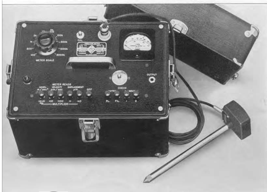
FIGURE 21. TYPE 761-A Vibration Meter, designed particularly for machinery vibration problems, covers the frequency range from 2 to 1000 cps (120-60,000 rpm).
