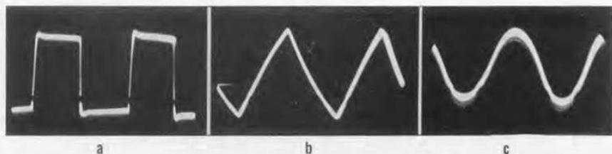
FIGURE 24. Illustrating the operation of the integrating circuits in the vibration meter (a) shows a square wave as transmitted by the amplifier when set for acceleration measurements, (b) shows the wave after one stage of electrical integration for velocity measurements, (c) shows the result of two stages of integration as used for displacement measurements. 28
